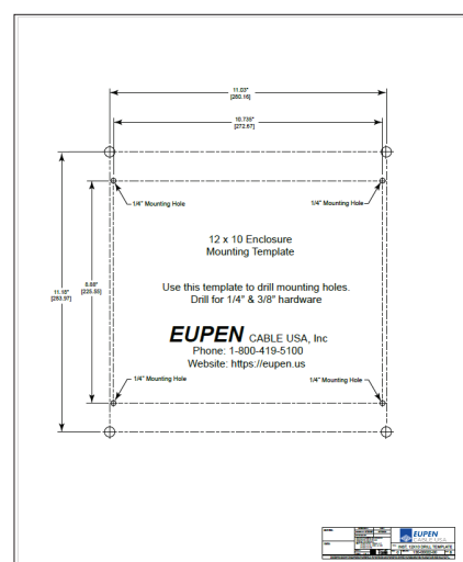
Wall Mount Drill Template
