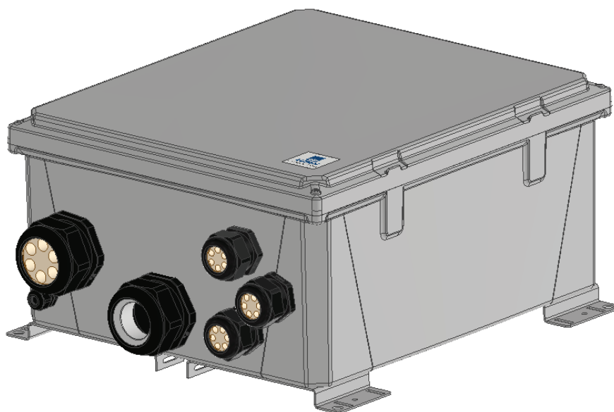
JB007 Junction Box Assembly
